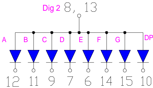
Common Anode
